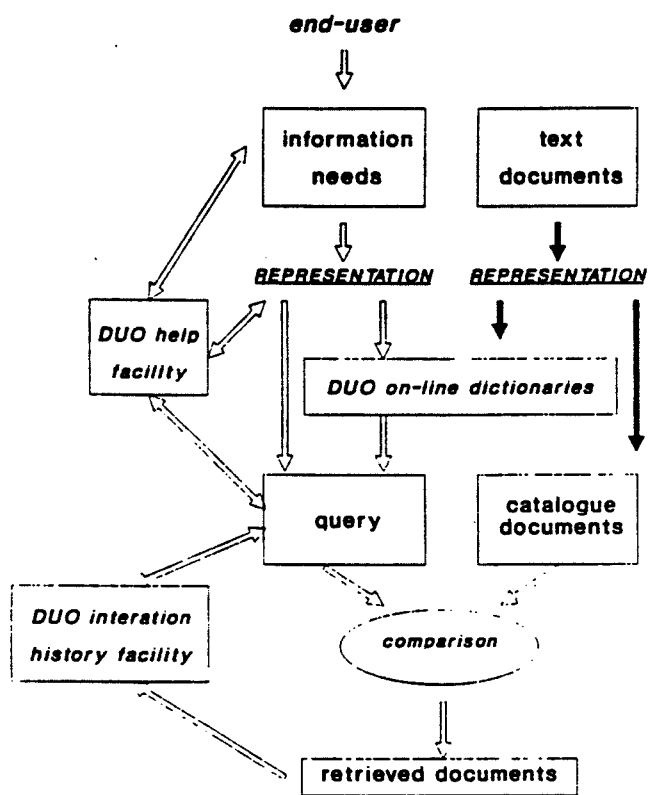
Figure 5: User-DUO Interaction
