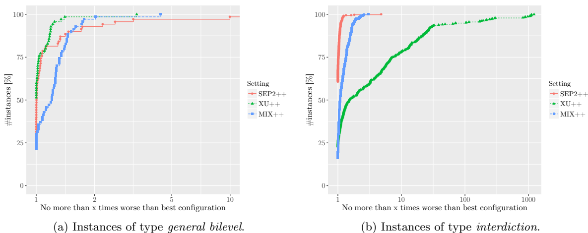
Figure 4: Effect of different ICs on the B&C performance. Performance profiles contain instances that could be solved to optimality by all three settings. FUB cuts and preprocessing are turned on.
