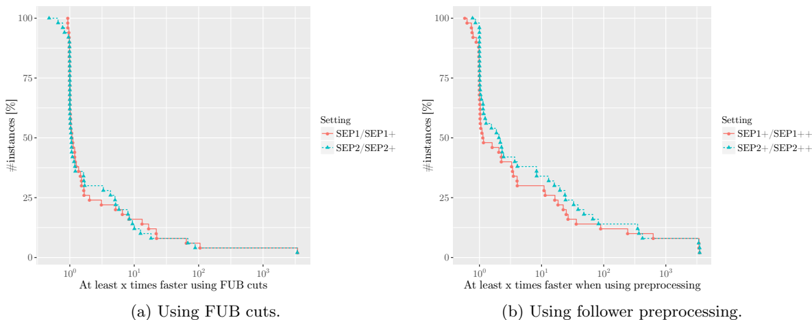
Figure 2: Speed-ups achieved by FUB cuts and follower preprocessing for the instance set DENEGRE .
