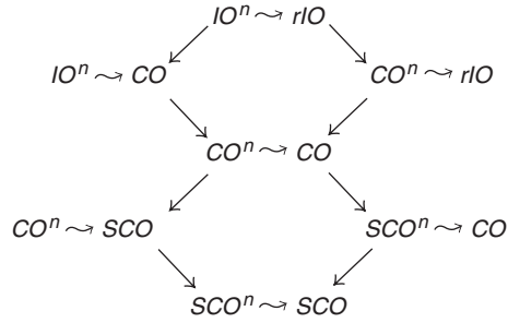
FIGURE 1. Lattice of impossibility results.
