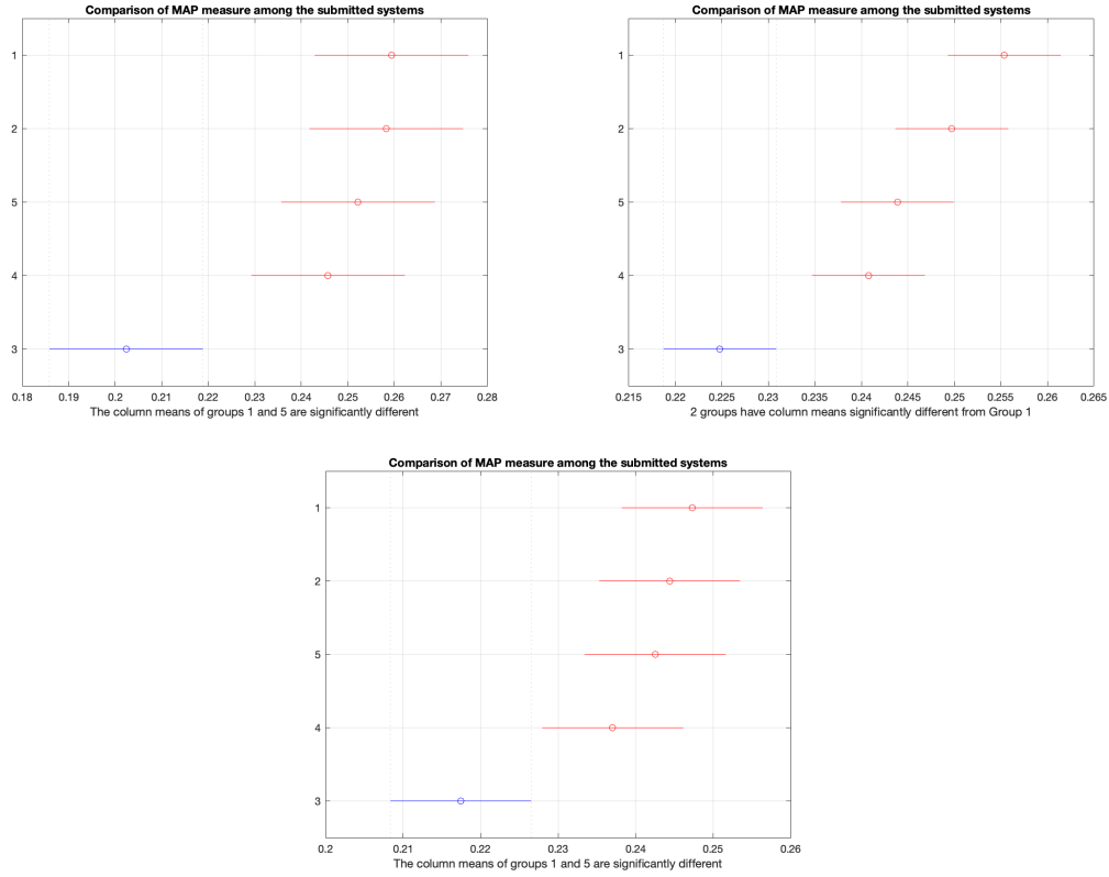
Figure 5: Average Precision
